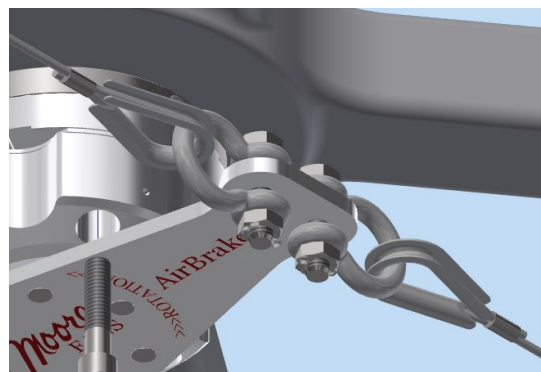
Figure 3. Installation of shackle
