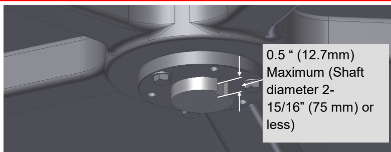
Figure 1. Maximum shaft extension.
