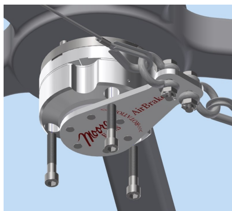
Figure 2. SF installation
