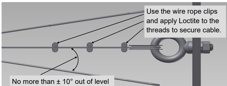
Figure 6. Restraining cable angle tolerance.
